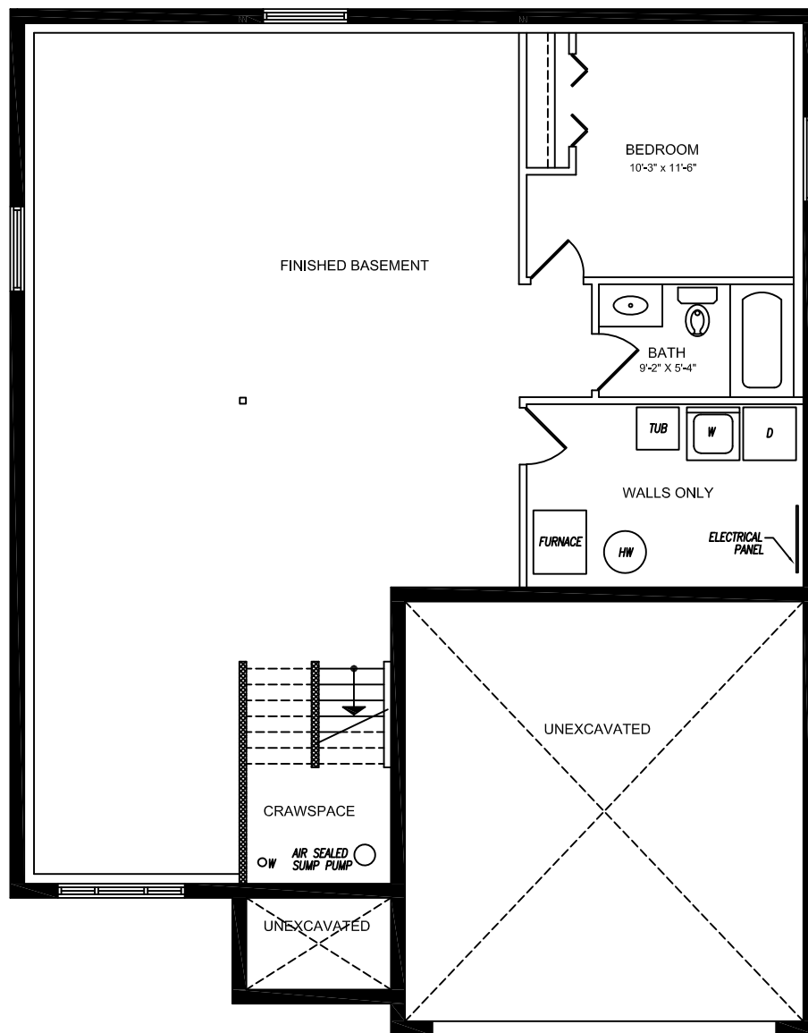
BASEMENT PLAN
